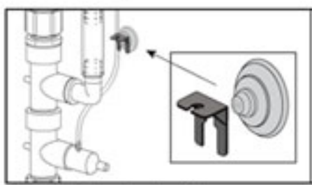
Airline Bracket with Suction Cup R440072
